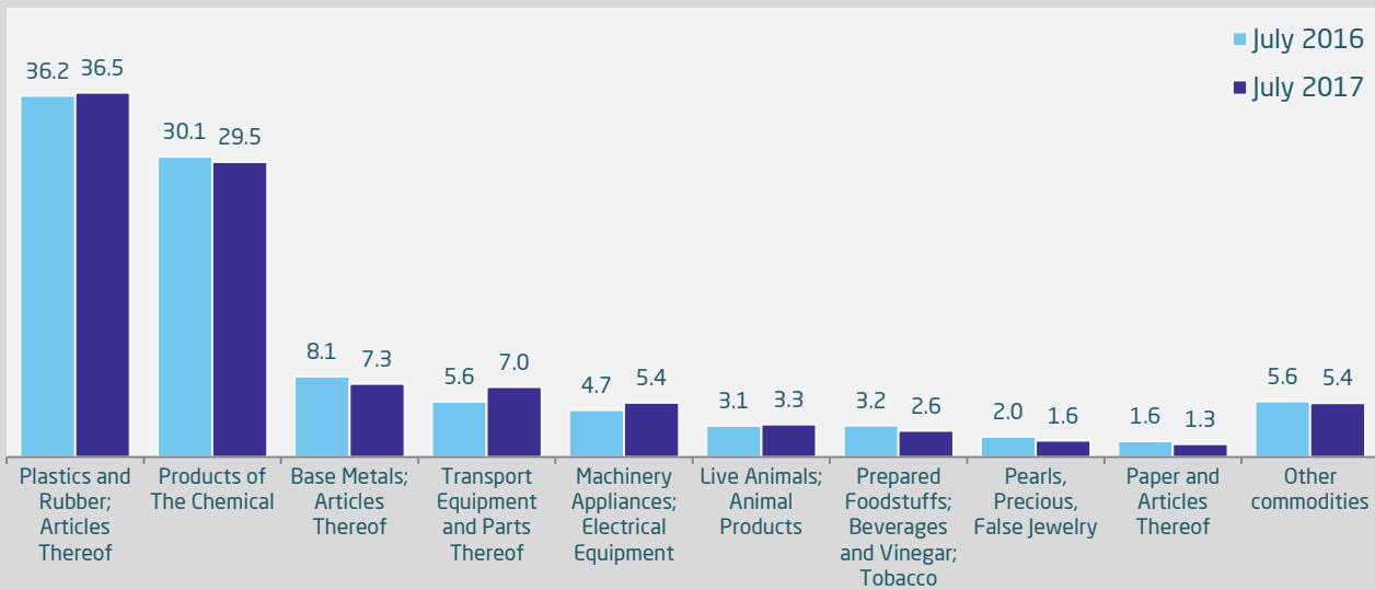
Change in Main Non-Oil Export Products, July 2017 (%)
